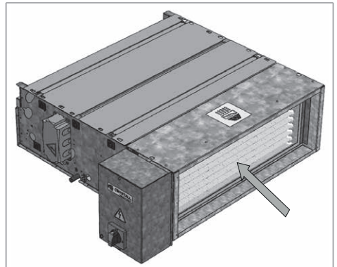
To apply the gasket to the electrostatic filter accessory within the lower internal side.
