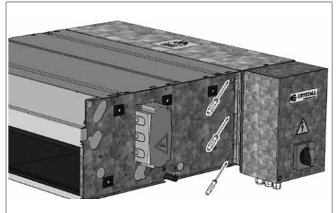
Screw the screws on both sides of the fan coil unit.
