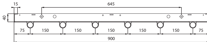
DS-ST28-2-105; 7 PIPES
