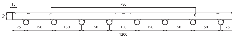
DS-ST28-2-135; 9 PIPES
