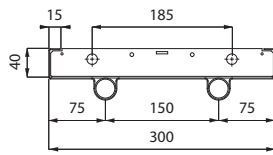
DS-ST28-2-045; 3 PIPES
