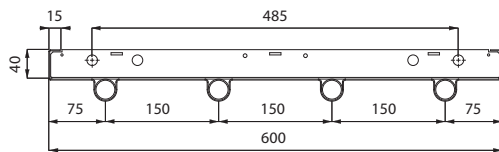
DS-ST28-2-075; 5 PIPES
