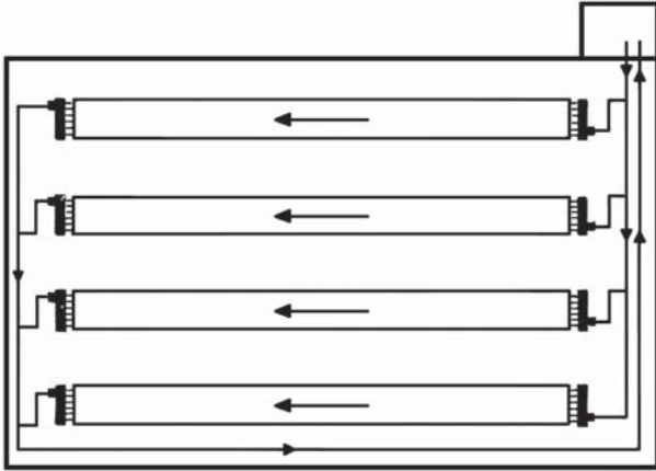
"B" HEADER COMPENSATED LINES
