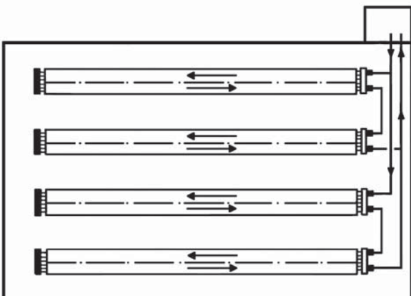
"D" HEADER LINES IN SERIES
