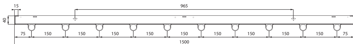
DS-ST28-2-150; 10 PIPES
