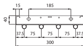
DS-ST18-4-060; 8 PIPES
