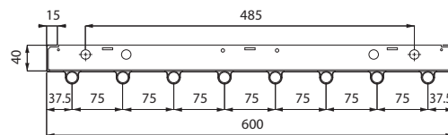
DS-ST18-4-090; 12 PIPES
