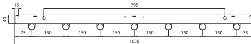
DS-ST28-2-120; 8 PIPES
