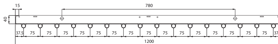
DS-ST18-4-120; 16 PIPES
