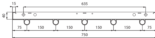
DS-ST28-2-090; 6 PIPES
