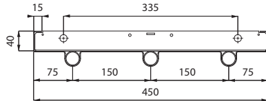
DS-ST28-2-060; 4 PIPES
