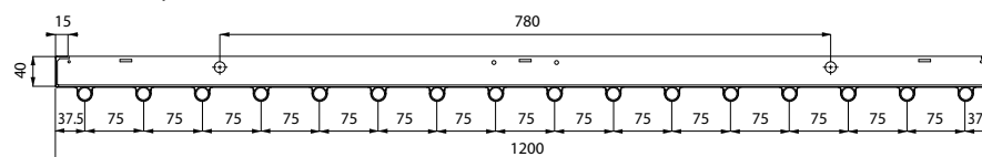
DS-ST18-4-120; 16 TUBI
