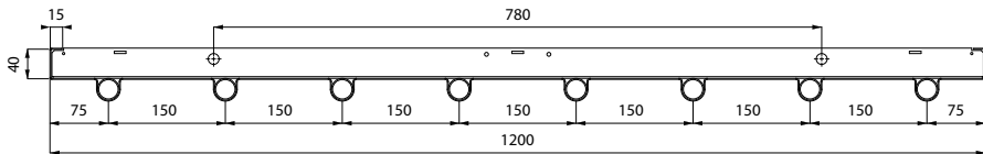
DS-ST28-2-135; 9 TUBES
