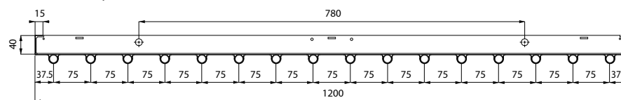
DS-ST18-4-120; 16 TUBES
