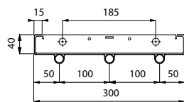
DS-ST18-3-060; 6 TUBES
