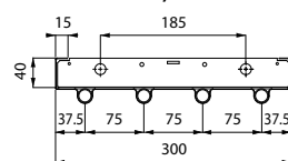
DS-ST18-4-060; 8 TUBES
