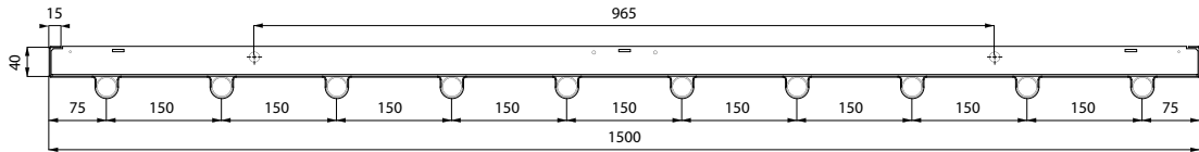
DS-ST28-2-150; 10 TUBES
