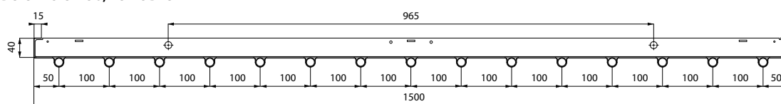
DS-ST18-3-150; 15 TUBES
