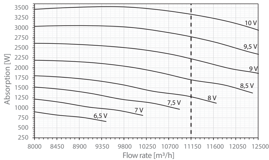
TZN 110 flow-rate-absorption curves
