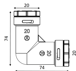
Articolo: SHRA01200120 x-light raccordo a gomito IR 20-20 mm
