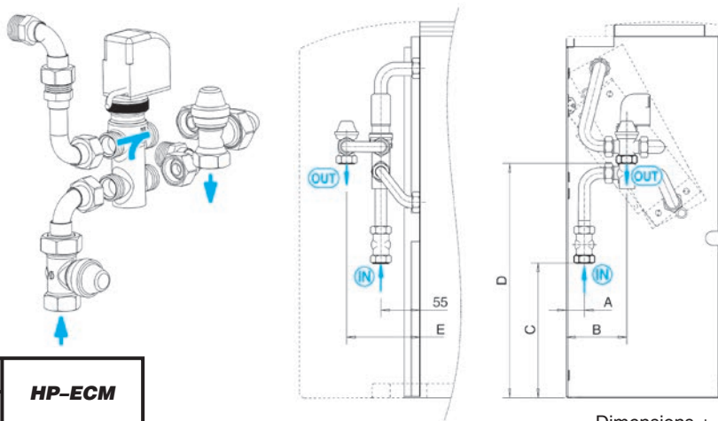
Dimensions ± 10 mm
