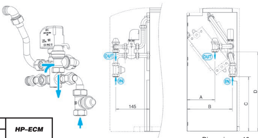
Dimensions ± 10 mm
