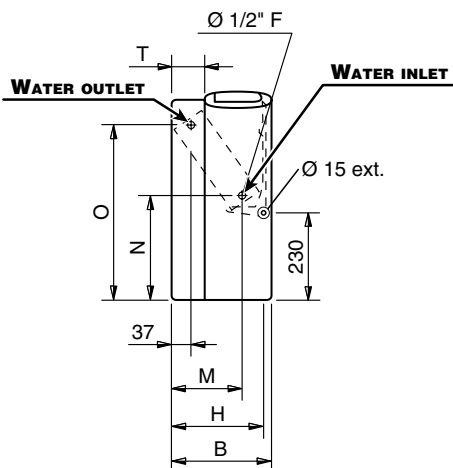
3 or 4 row coils
