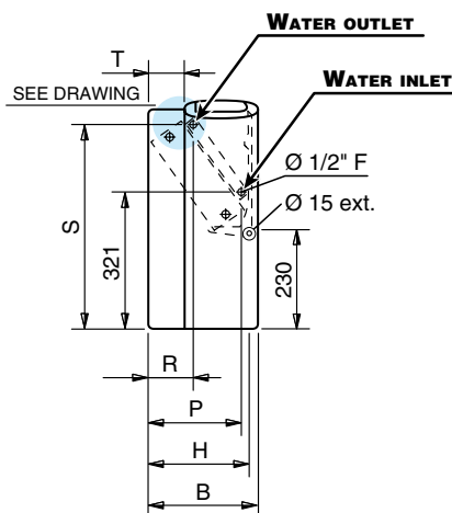
Heating additional coil (1 or 2 rows)
