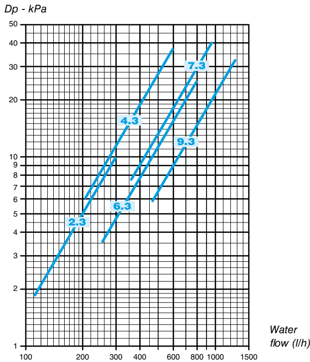
3 row coil
