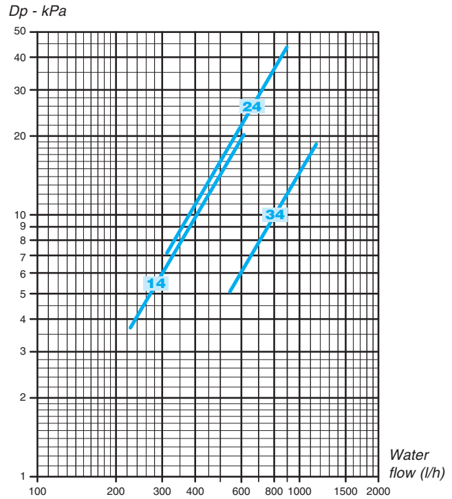
4 row coil
