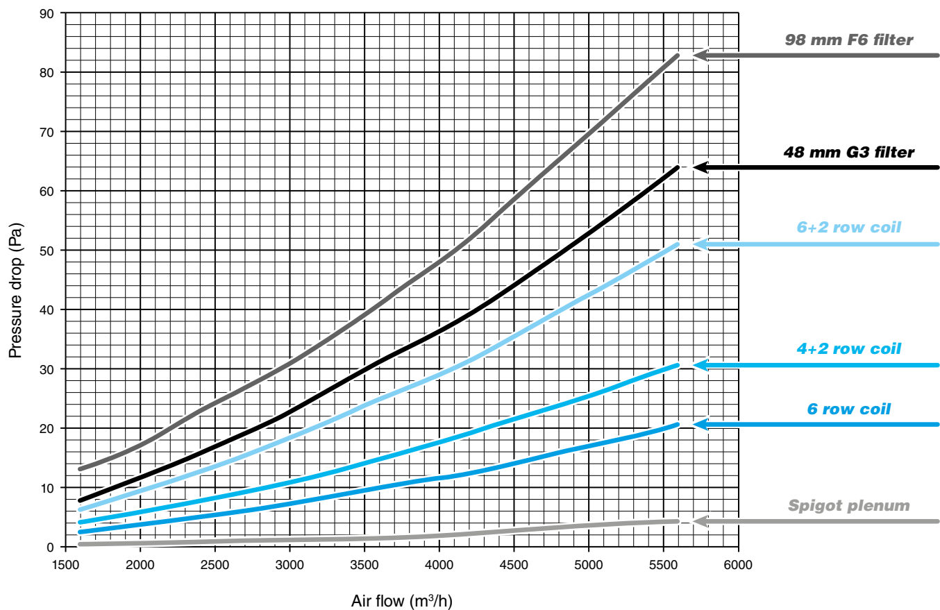
Pressure drop for DFCL 6 (Dp)
