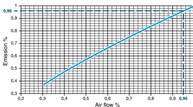
Diagram 2 – Heating emission
