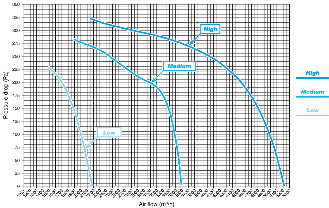
Available pressure for DFCL 64 (with 4 row coil)
